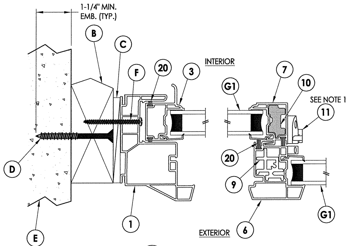
1 2 HORIZONTAL CROSS SECTION 2X Buck Masonry Construction
